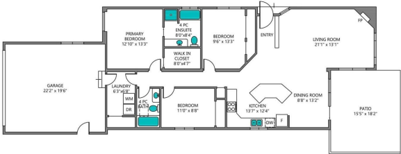
MAIN LEVEL 1,510 SQ. FT.
